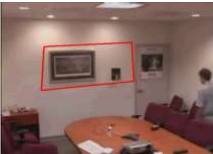
Object Missing
